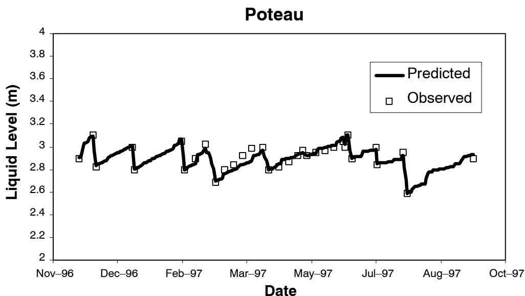
Figure 3. Observed and predicted lagoon elevations for the facility located in Poteau from 11 November 1996 to 22 September 1997.
