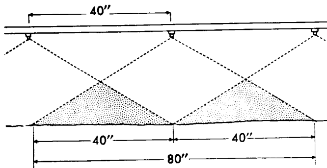
Flooding Nozzle Spray Overlap (100 Percent)
