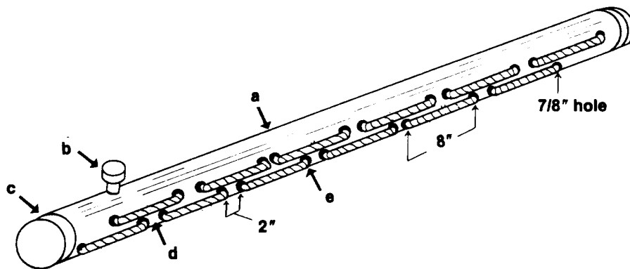
Figure 11.3. Typical ropewick applicator showing the components assembled. Materials are (a) 3-inch PVC pipe; (b) capped fill spout – PVC; (c) end cap – PVC; (d) wick of ½-inch diameter soft braided nylon marine rope; (e) rubber bushing (for ½-inch rope) with compression cap.
