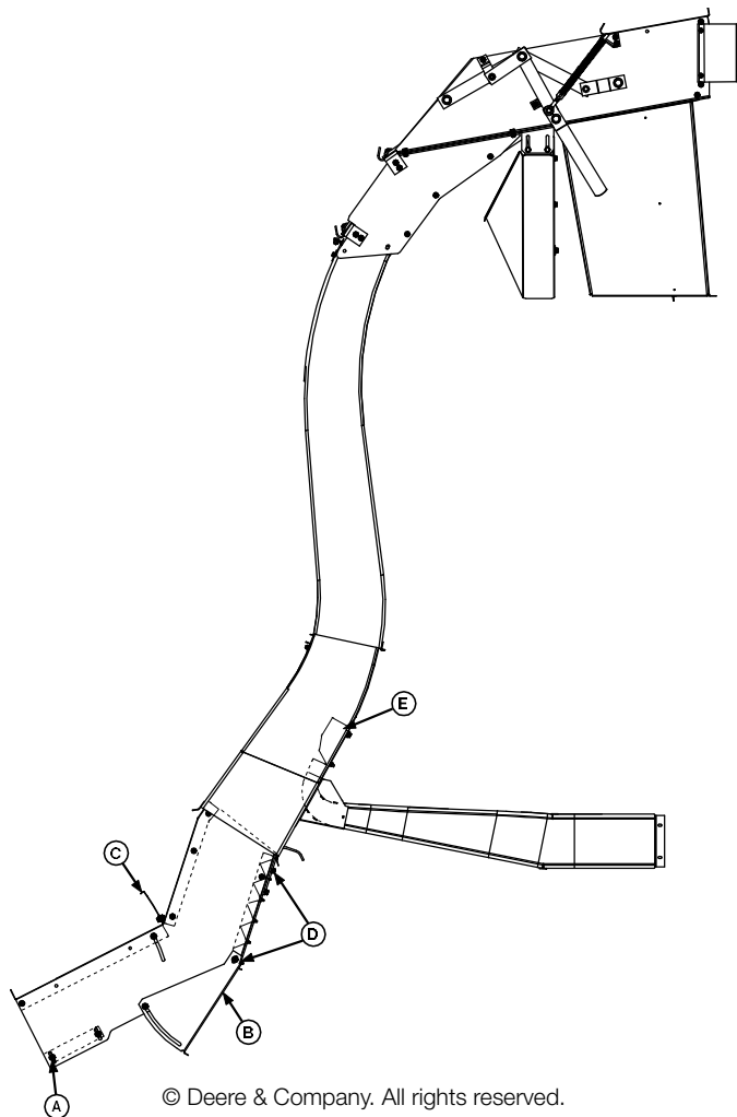
Schematic of main cotton conveying duct used on John Deere 7460 stripper harvesters (Courtesy of John Deere): A – Lower Front Separation Duct Panel; B – Lower Separation Duct Door; C – Door; D – Separator Angles; and E – Vanes.
