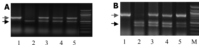
Figure 5. Discovered two copies of Lr34 in Duster. (A) Duster in lanes 3 to 5 shows heterogeneous band patterns for Lr34E11 . Lane 1, 2174, and lane 2, Billings, represent the resistant allele and the susceptible allele, respectively. (B) Duster in lanes 3 to 5 shows heterogeneous band patterns for Lr34E12 . Lane 1, 2174, and lane 2, Billings, represent the resistant allele and the susceptible allele, respectively.
