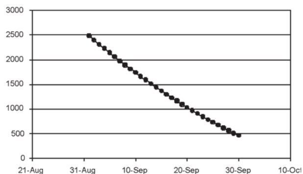
Figure 1. Wheat fall forage yield as affected by planting date at Lahoma, Okla. from 1991 to 1999.
